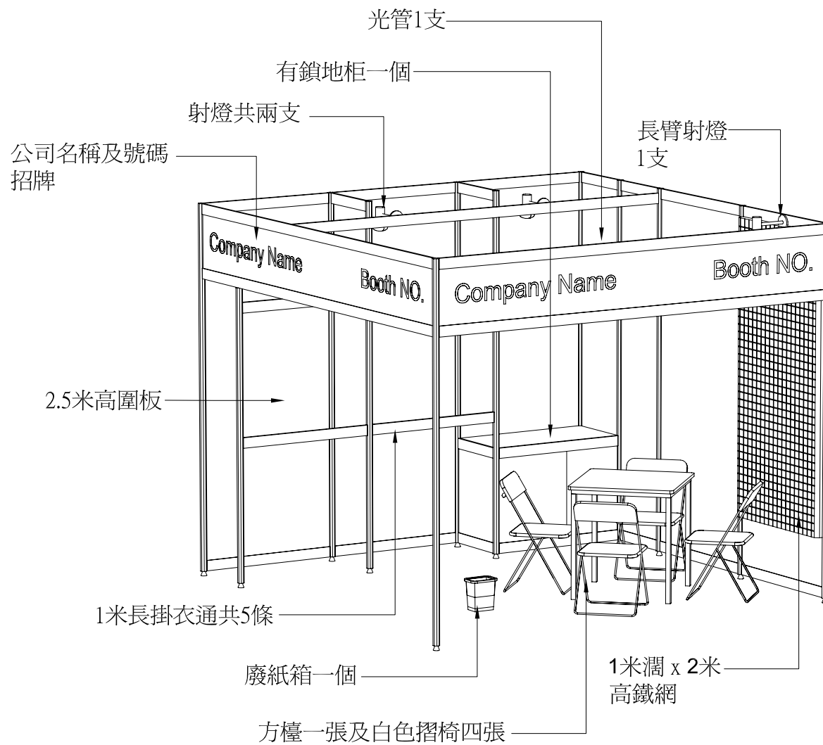
Perspective View
