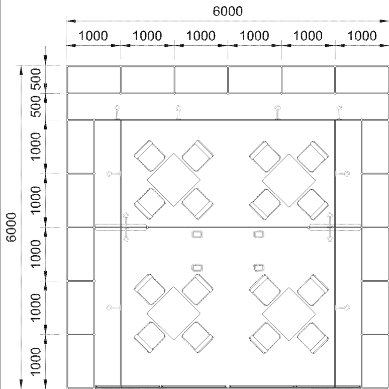
Plan View
